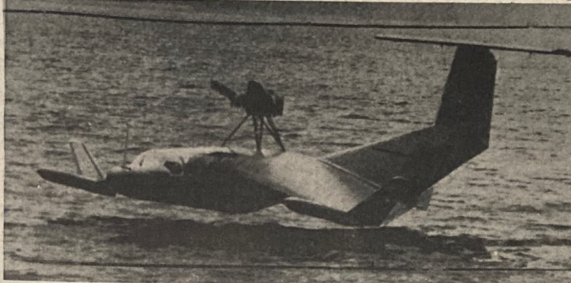
SUCCESSFUL TESTS on the 'Airfoil' were recently completed at Lake Konstanz, Germany. The flying boat, designed by German aerodynamics expert Alexander Lippisch, has specially designed wings that use the 'ground effect' for increase of lift. It is made of fiber glass.
